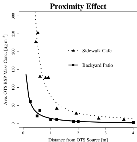
FIGURE (3): Overall average outdoor tobacco smoke (OTS) respirable suspended particle (RSP) mass concentrations across all instruments as a function of proximity to the OTS source, calculated using levels measured during experiments on a backyard patio and two sidewalk cafés for which source proximity was recorded precisely (see E1–E4 and OP1–OP3 in Table 3). Background RSP levels were subtracted from all measurements. The backyard patio experiments used smolder-smoked cigarettes in an area shielded by fences and trees. The sidewalk café experiments used smolder- or human-smoked cigarettes.
