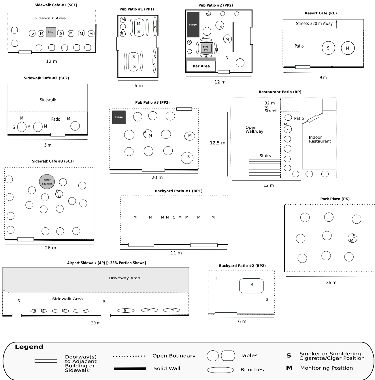
FIGURE (1): Rough schematic diagrams of patios and sidewalks where outdoor tobacco smoke (OTS) particle levels were monitored in proximity to smokers or burning cigarettes. All the patios had at least an open roof and many were open on three sides. Broken lines represent open boundaries, and solid lines indicate a surrounding wall or an adjacent building. Tables and benches are represented by circles or ovals and rectangles indicate doorway(s) to buildings or an opening in the wall or fence surrounding a patio. The approximate positions of active smokers and monitors during one or more visits are indicated by the letters "S" and "M", respectively. See Table 4 for dimensions and other characteristics of each OTS monitoring location.
